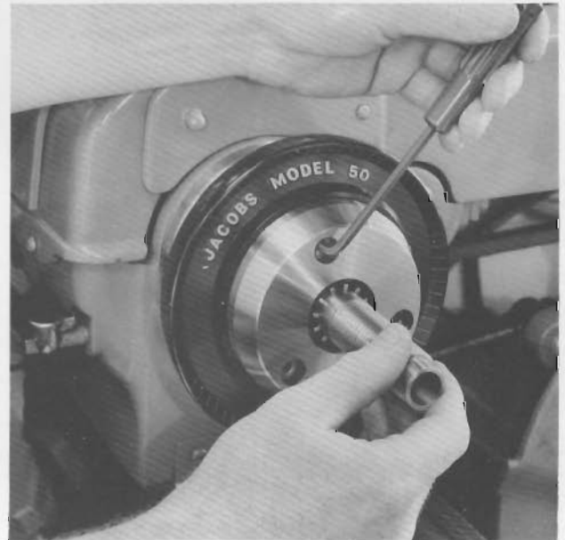
Model 50 Collet Chuck
